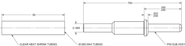
Dimensions are in inches.
